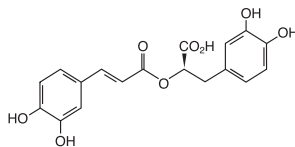
Rosmarinic Acid
